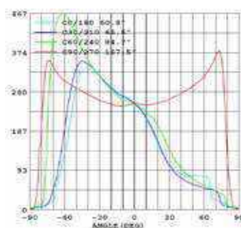
Illumination Curve
